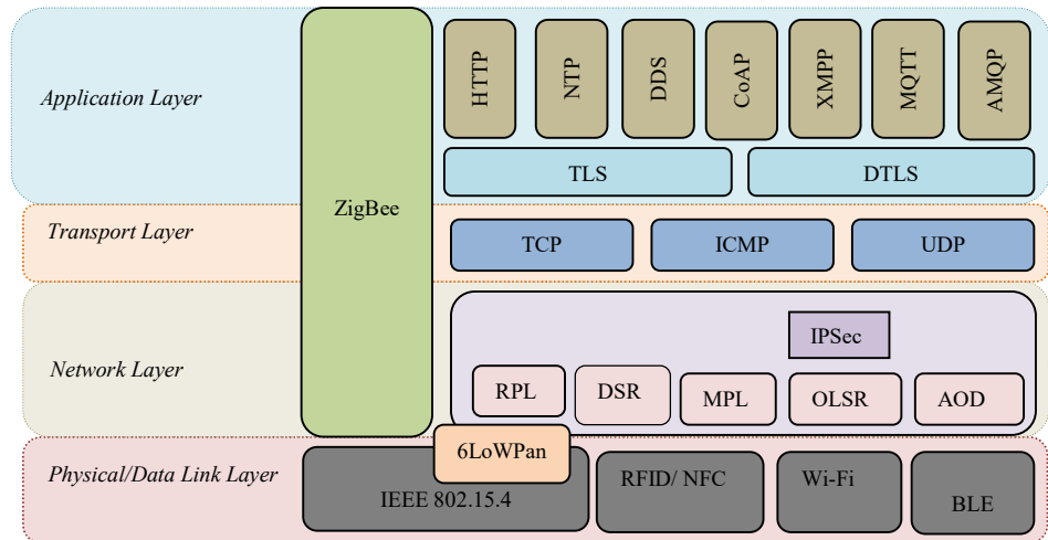
Figure11: IoT protocols
